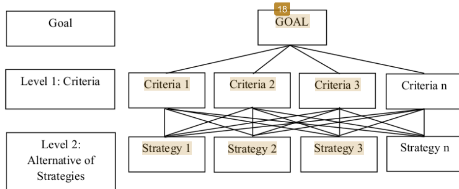
Figure 2. AHP Hierarchy Model (Saaty, 1993)
